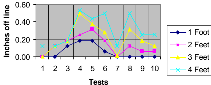
Deviations of Joined-Axle Robot with Matched Motor
