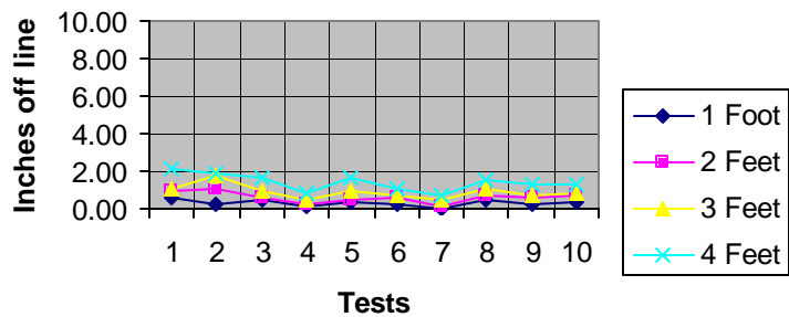
Deviations of Joined-Axle Robot with Non-Matched Motors
